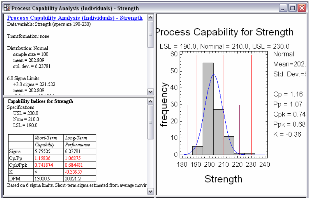
Figure 15-4. Process Capability Analysis Window
