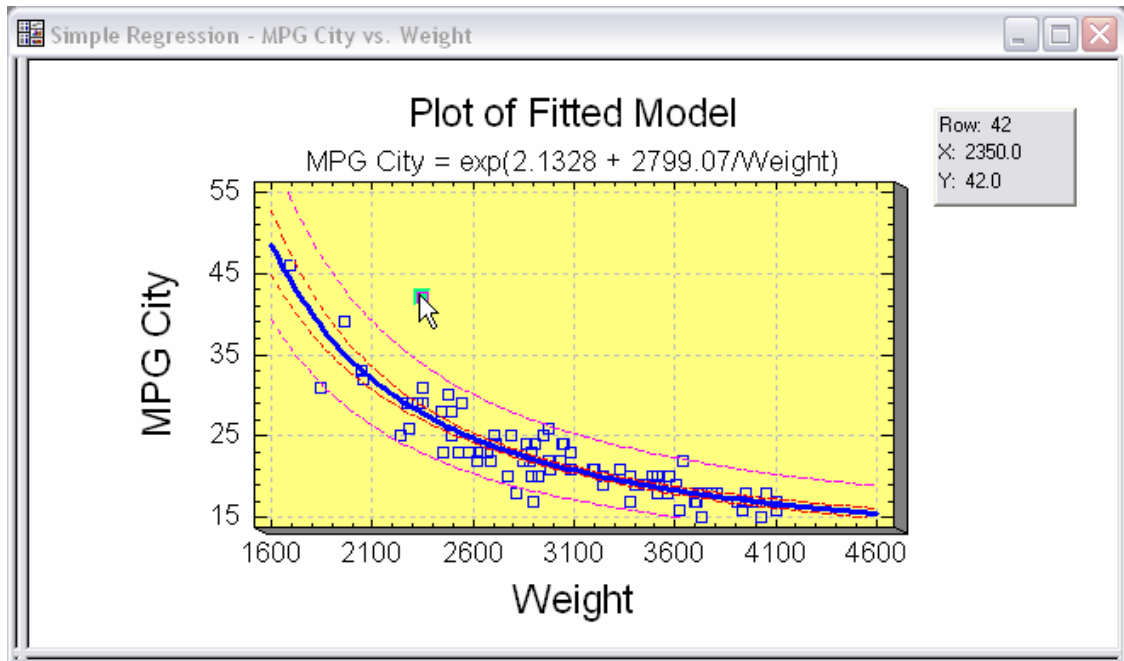
Figure 4-27. Displaying Information about a Selected Point
