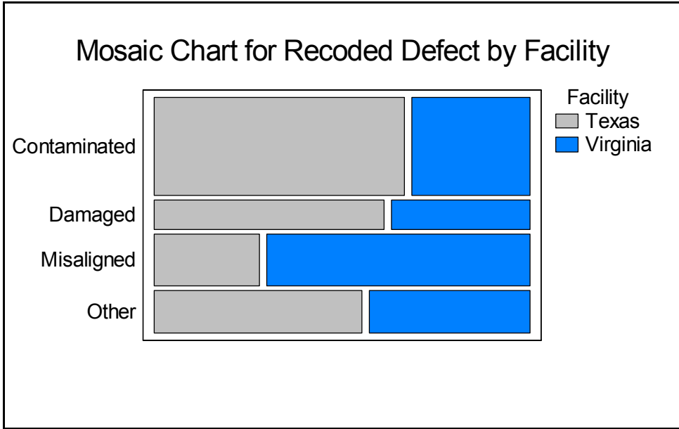
Figure 14-16. Mosaic Plot for Recoded Data
