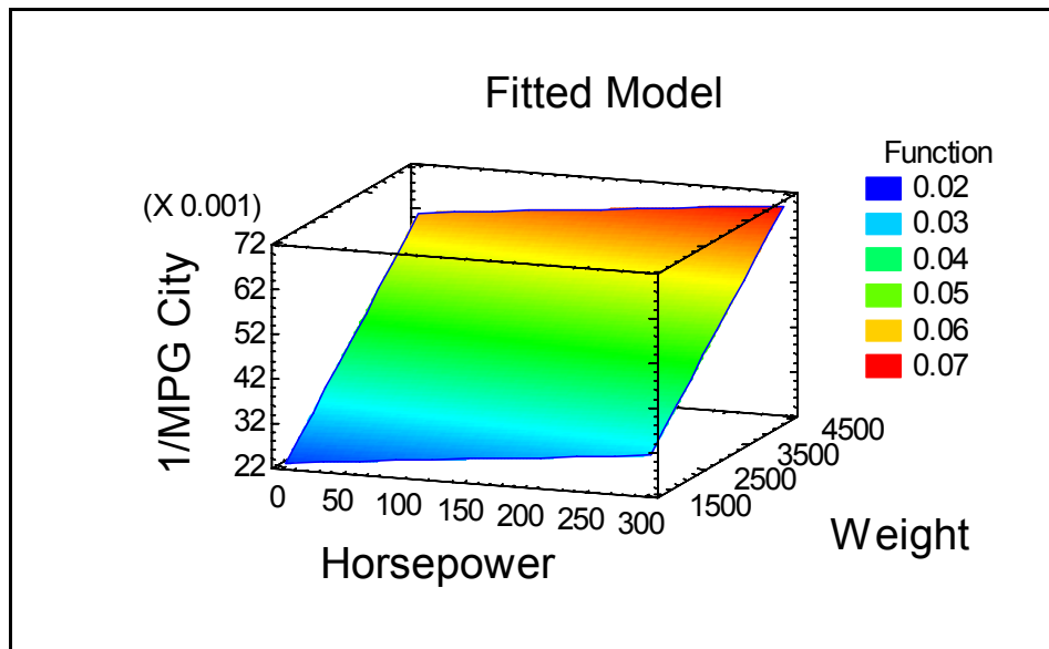
Figure 13-20. Plot of Fitted Model
