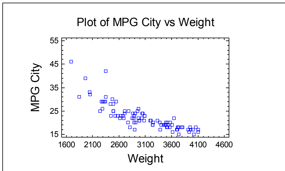
Figure 3-1. X-Y Plot of Miles per Gallon in City Driving versus Weight in Pounds
