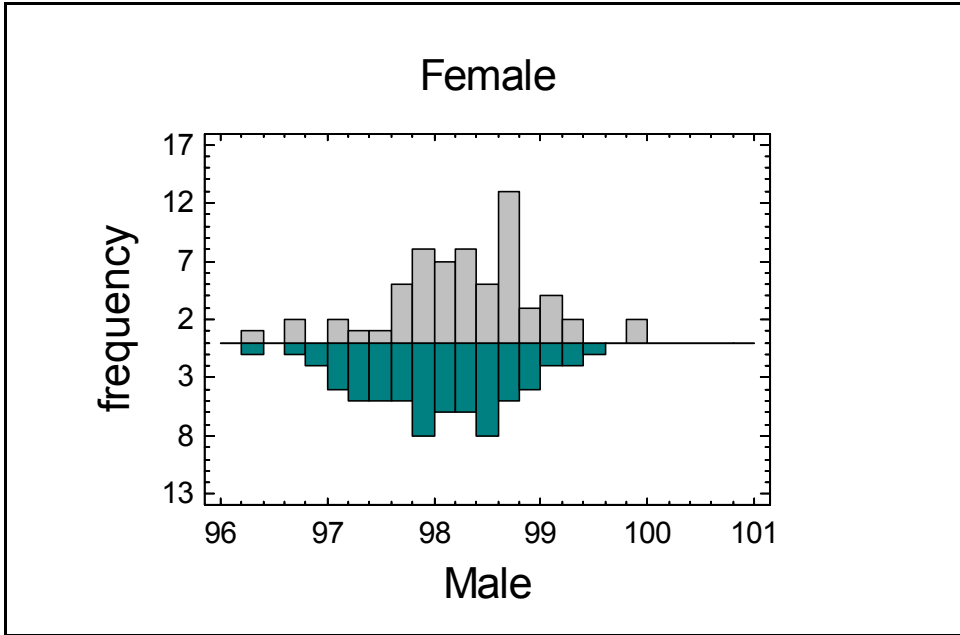
Figure 11-4. Dual Frequency Histogram
