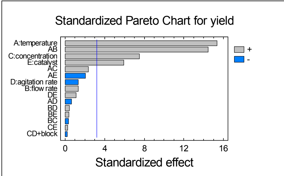
Figure 16-14. Standardized Pareto Chart
