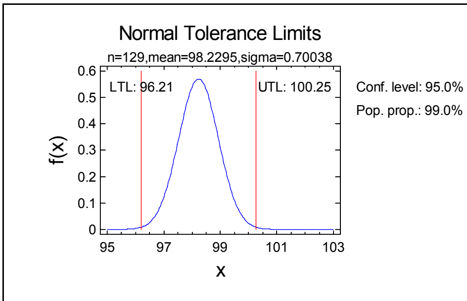
Figure 10-27. Tolerance Plot
