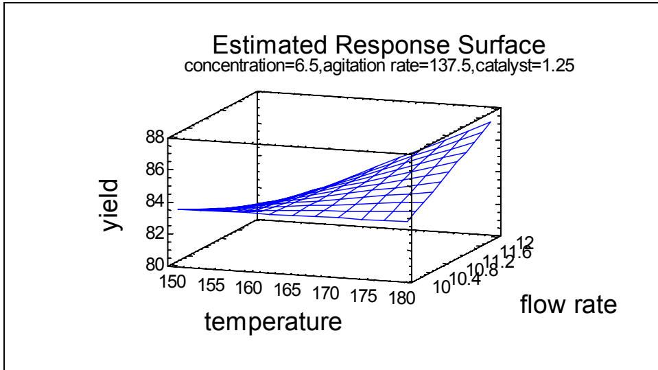
Figure 16-21. Response Surface Plot
