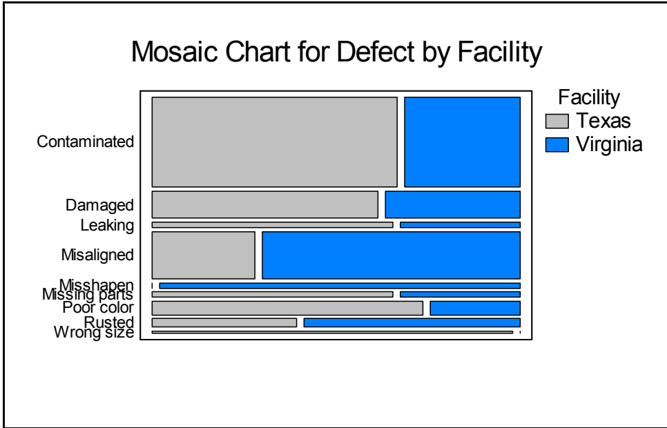
Figure 14-12. Mosaic Plot
