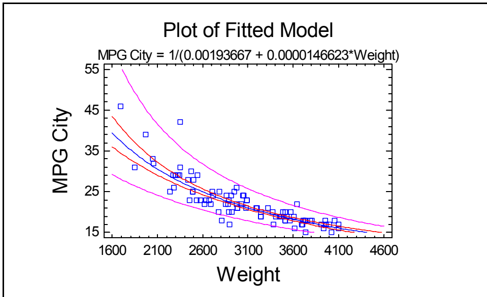
Figure 13-10. Fitted Reciprocal-Y Model
