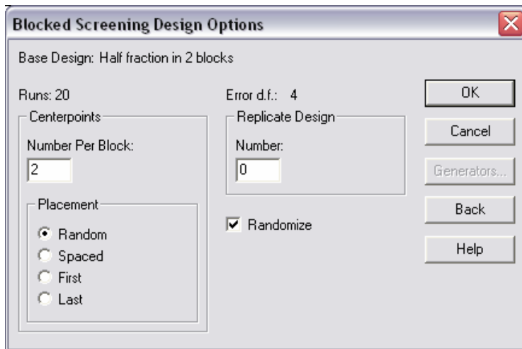
Figure 16-8. Design Options
