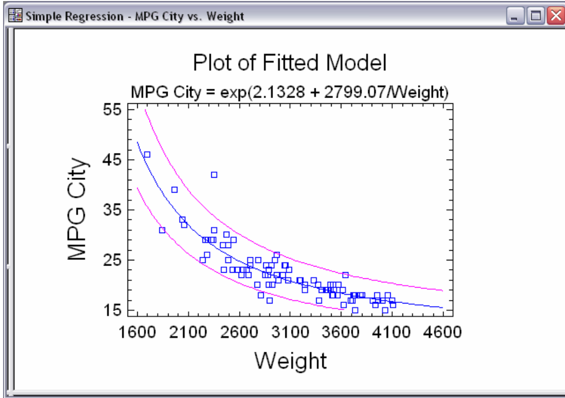
Figure 3-14. Fitted Model Plot Without Confidence Limits
