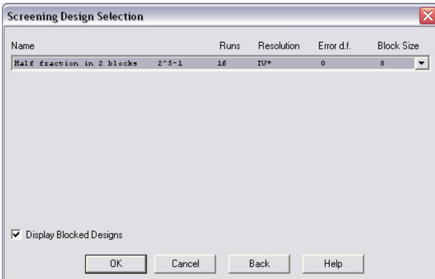
Figure 16-7. Design Selection
