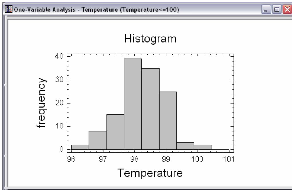
Figure 10-13. Frequency Histogram with Default Classes
