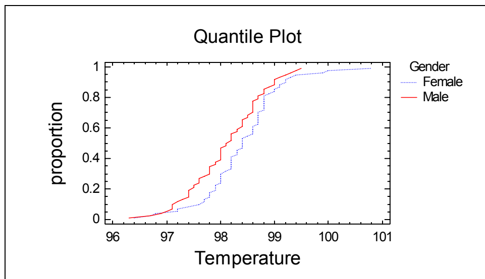
Figure 11-9. Side-by-Side Quantile Plots
