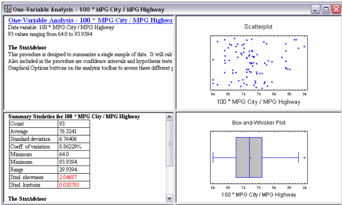
Figure 2-11. One-Variable Analysis of Transformed Data
