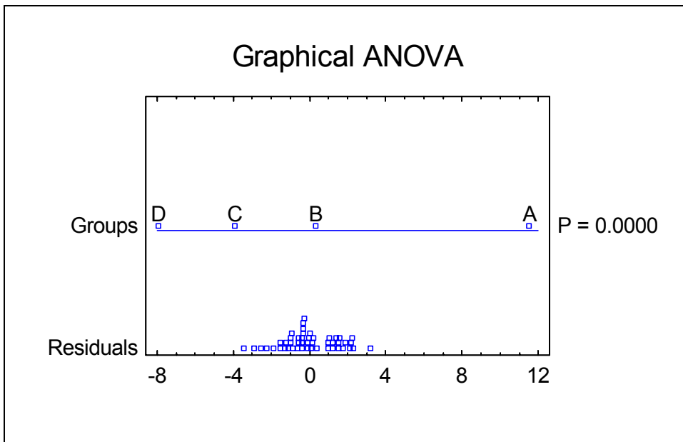
Figure 12-8. Graphical ANOVA
