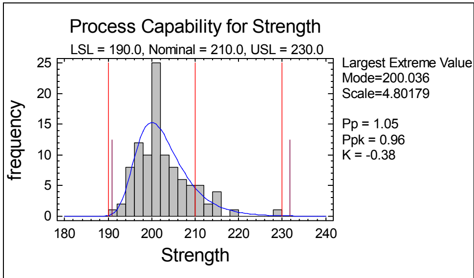
Figure 15-10. Fitted Largest Extreme Value Distribution
