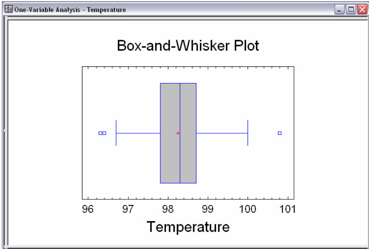
Figure 10-7. Box-and-Whisker Plot for Body Temperatures
