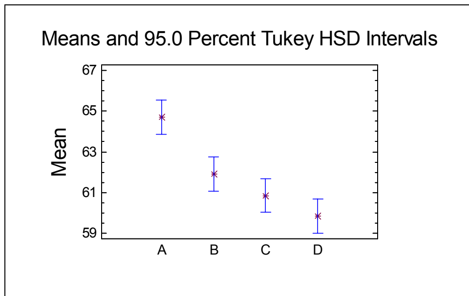
Figure 12-9. Means Plot
