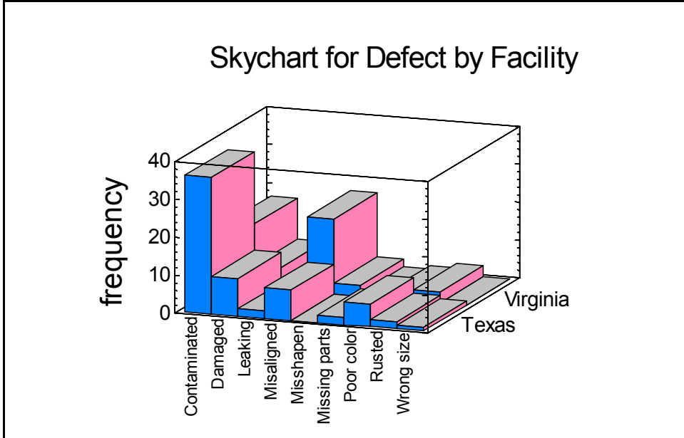
Figure 14-13. Three-Dimensional Skychart
