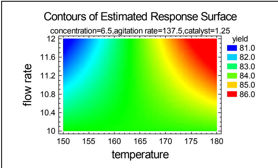
Figure 16-25. Contour Plot of Response Surface
