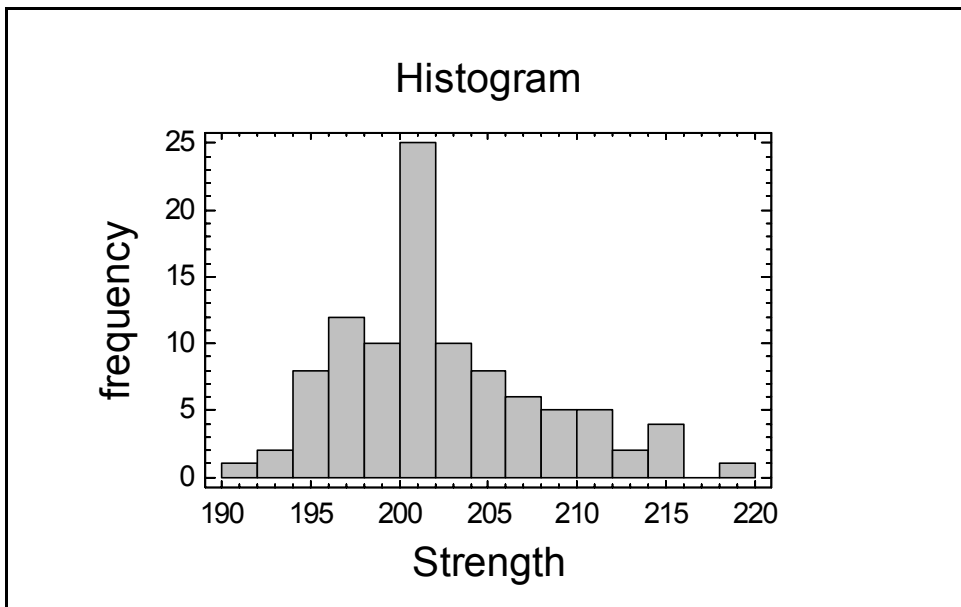
Figure 15-2. Frequency Histogram
