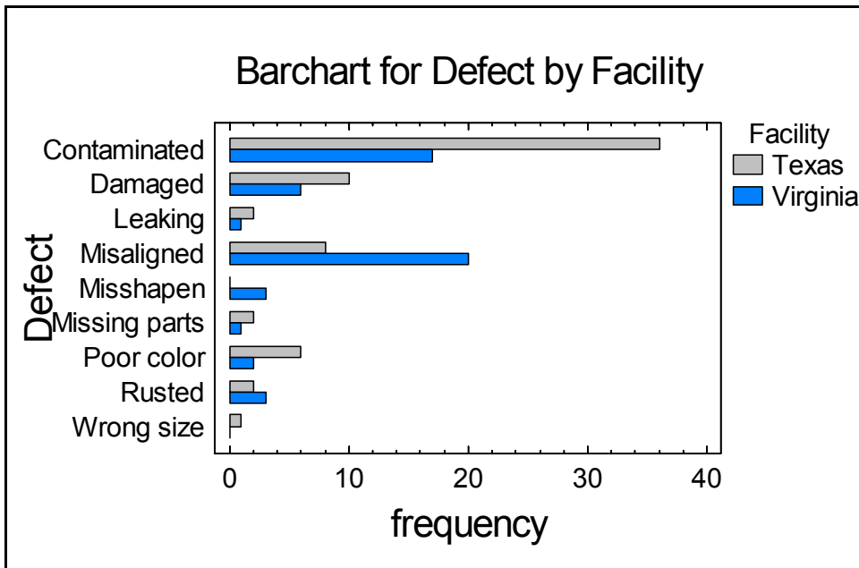
Figure 14-11. Clustered Barchart
