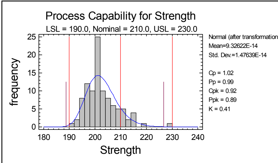
Figure 15-13. Capability Plot after Box-Cox Transformation
