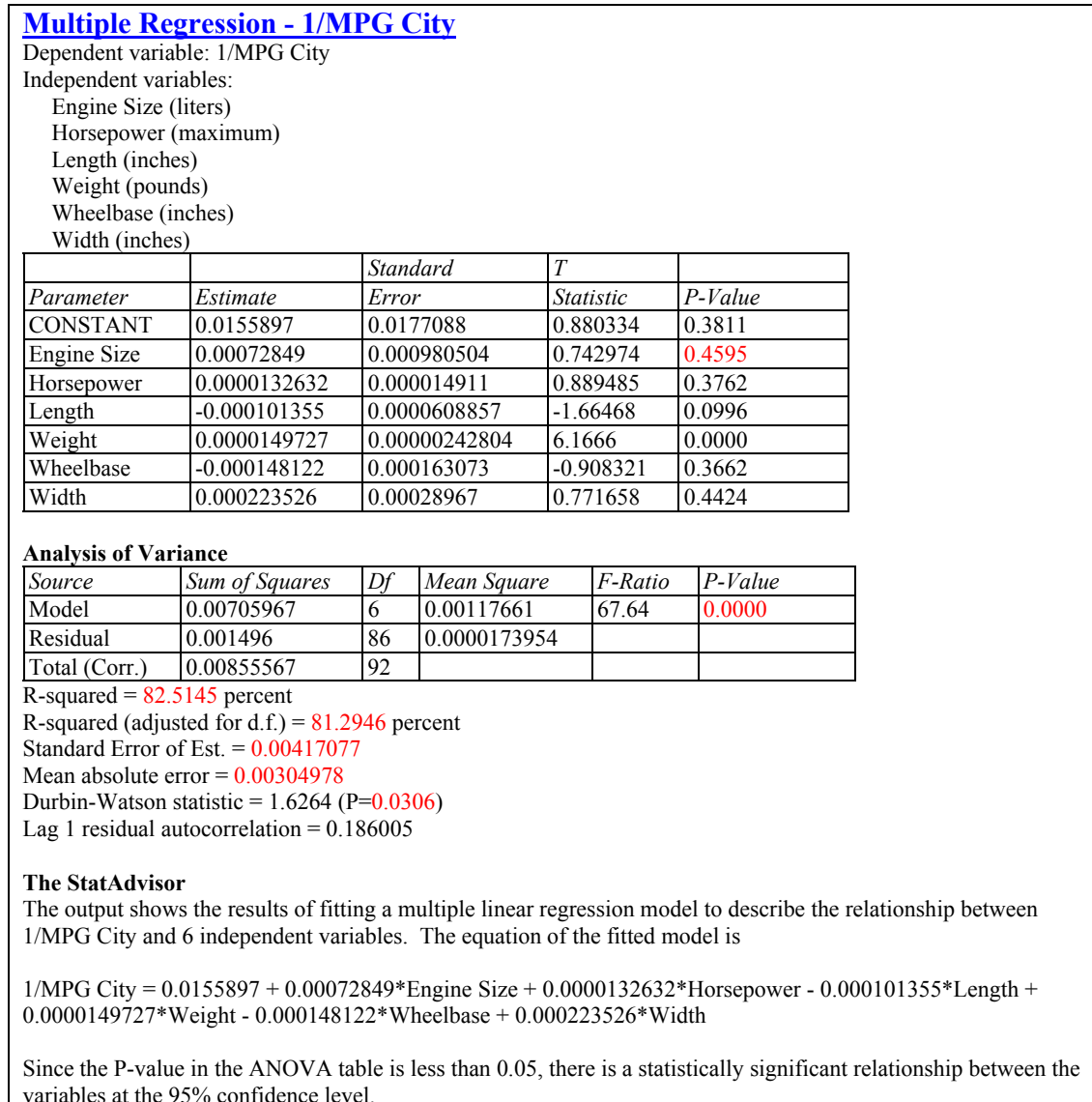
Figure 13-14. Multiple Regression Analysis Summary with 6 Predictor Variables
