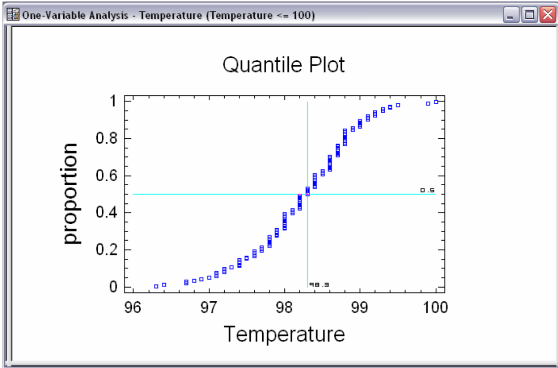
Figure 10-18. Quantile Plot
