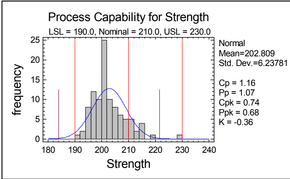
Figure 15-5. Capability Plot with Normal Distribution
